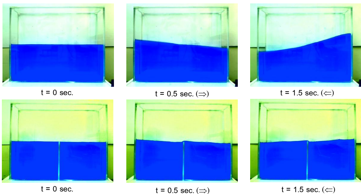
Fig. 6. Sequential images of the experimental surface wave inside the tank with and without a baffle at the initial condition and move to right (=>) and left (<=), respectively.
