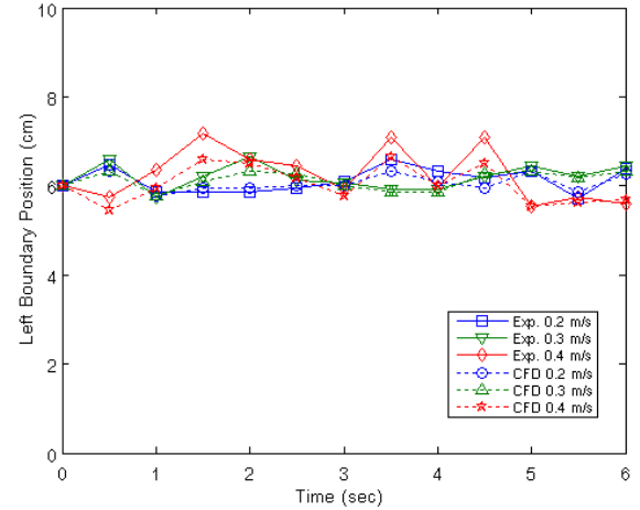
Fig. 11 Plot of the surface heights on the left wall of tank with baffle vs. time comparing CFD to experiments of the water 1/4 tank volume.
