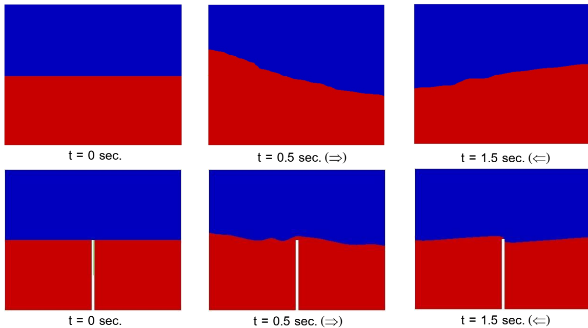
Fig. 7. Sequential images of the FVM surface wave inside the tank with and without a baffle at the initial condition and move to right (⇒) and left (⇐), respectively.
